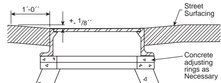
Adjusting utility cover level with road.
